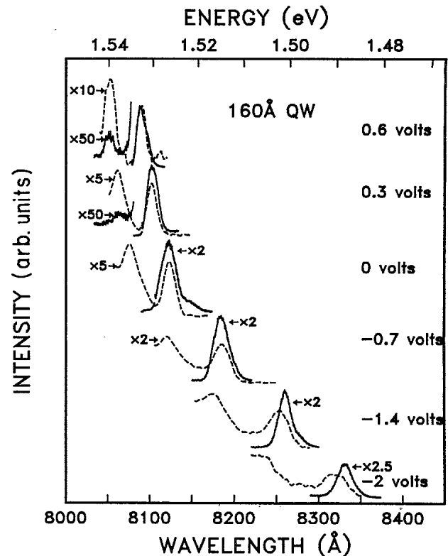
FIG. 2. Photoluminescence and photocurrent spectra at different external voltages. The measurements were done at the same temperatures as in Fig. 1. The spectra are displaced vertically with respect to each other for clarity; the high-energy peaks correspond to 1e1hh , while those at lower energies correspond to 1e1lh excitons. The vertical scale of some of the spectra has been enhanced by the factors indicated with arrows beside the spectra.
