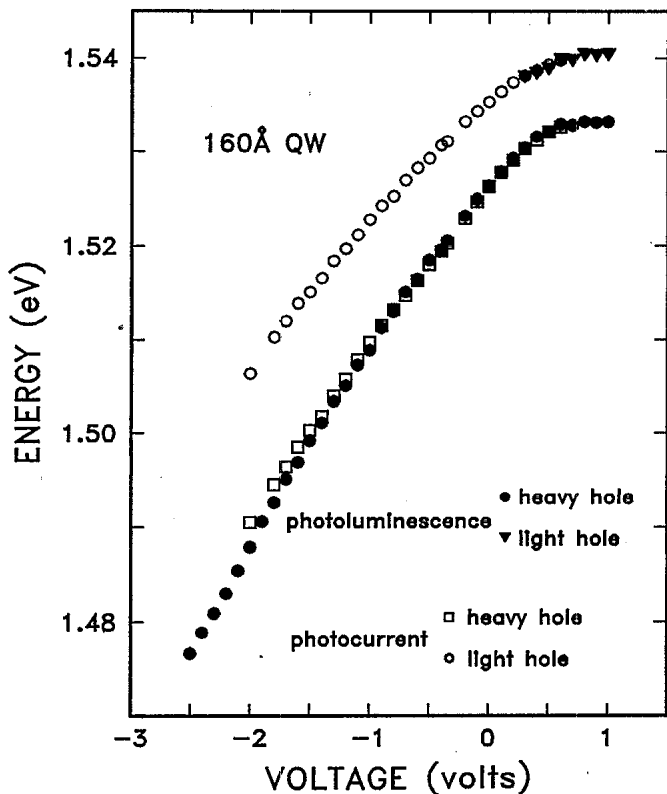
FIG. 3. Energies of the excitonic peaks as a function of applied external voltage obtained by photoluminescence (●, heavy hole; ▼, light hole) and photocurrent (□, heavy hole; ○ light hole) spectroscopy. Note that for voltages smaller than \sim -1 V, both structures shift below the bulk GaAs band edge.
