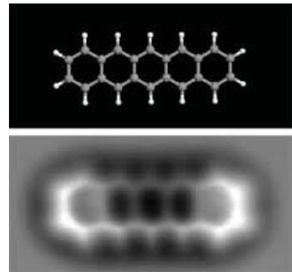
Pentaceno: Atomic Resolution AFM image
