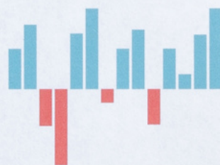
Bar Chart
