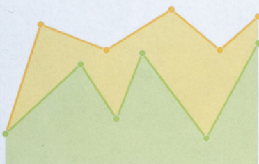
Line Chart
